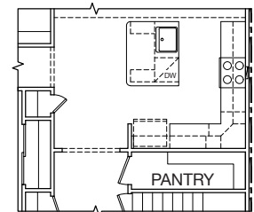
ALTERNATE KITCHEN
